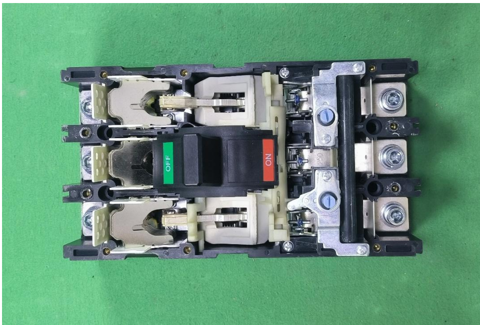
Internal view, GYCM8RT-630M, 3P, 320 A, 40 °C
