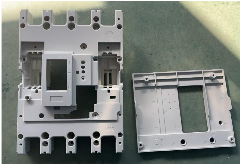
Internal view of white cover, 4P
