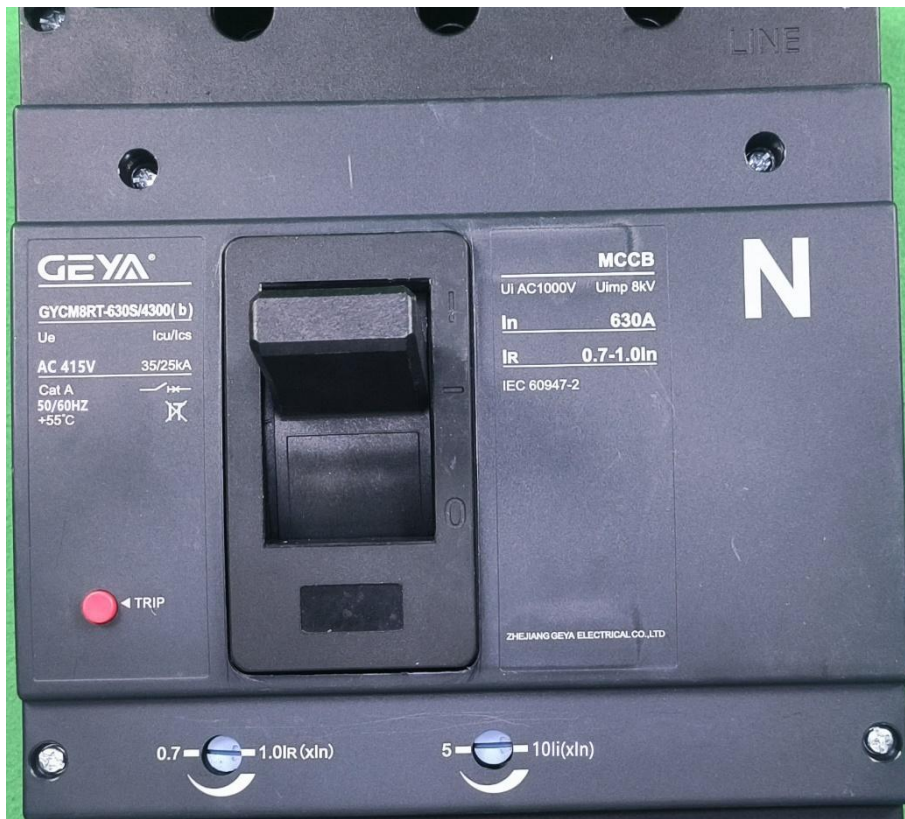
GYCM8RT-630S/4300(b), 630 A, 4P
