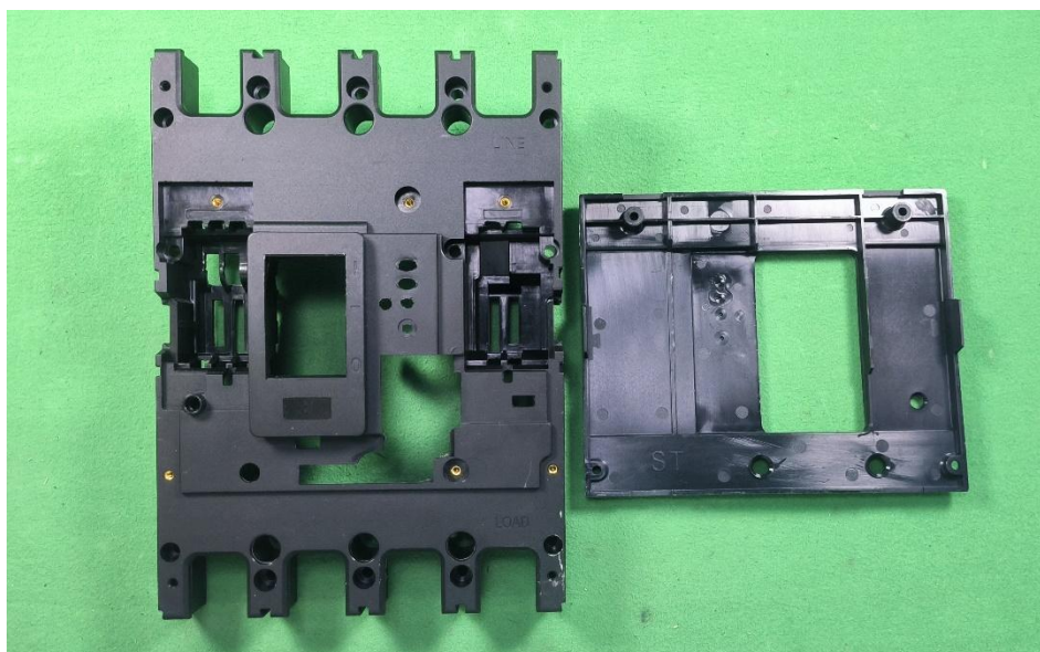
Internal view of black cover, 4P
