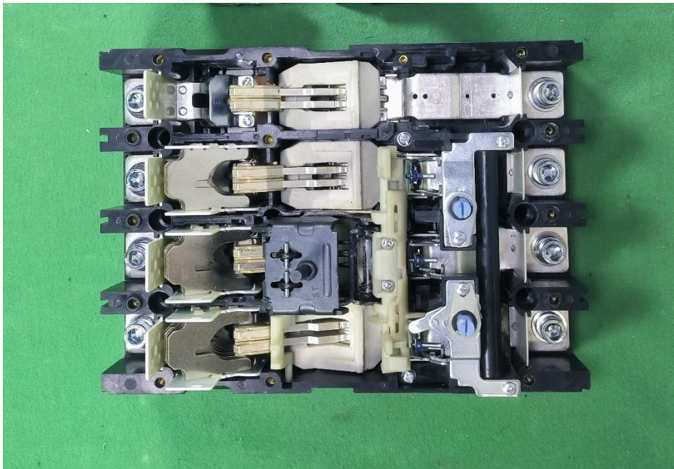
Internal view, GYCM8RT-630S, 4P, 630 A, 55 °C
