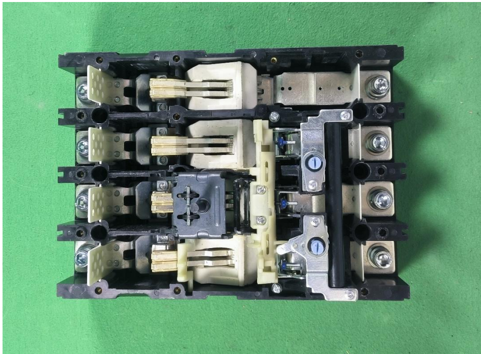
Internal view, GYCM8-630H, 4P, 400 A, 55 °C
